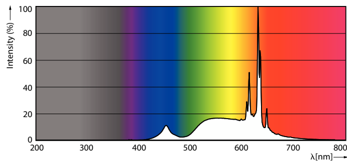
Spectral Power Distribution Colour - MAS VLE LEDBulb DT3.4-40W E27 927A60CL G
