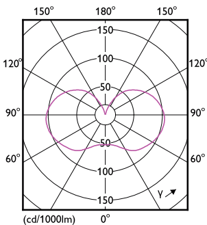
Light Distribution Diagram - MAS VLE LEDBulb DT3.4-40W E27 927A60CL G
