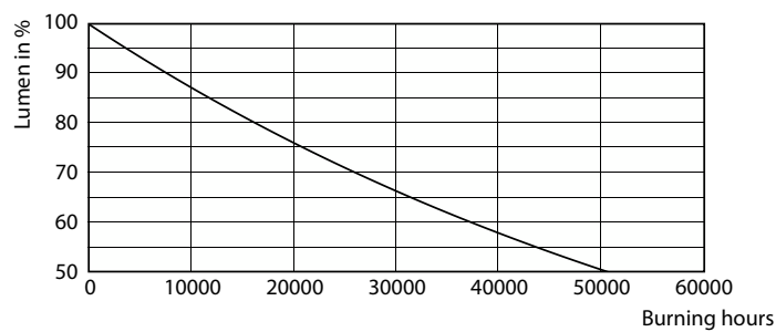
Lumen Maintenance Diagram - MAS VLE LEDCandleDT3.4-40W E14927BA35CLG
