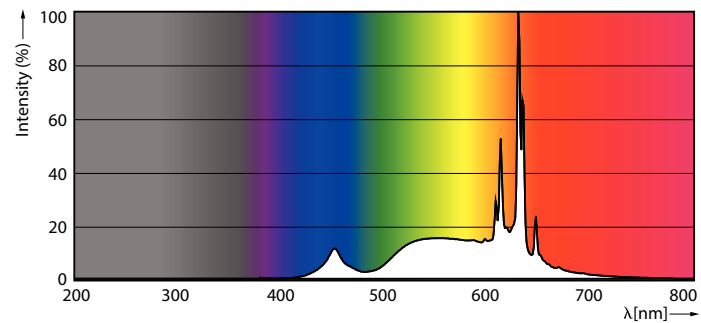
Spectral Power Distribution Colour - MAS VLE LEDCandleDT3.4-40W E14927BA35CLG
