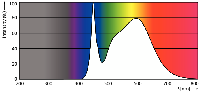
Spectral Power Distribution Colour - 14.5T8/COR/48-840/MF21/G 10/1
